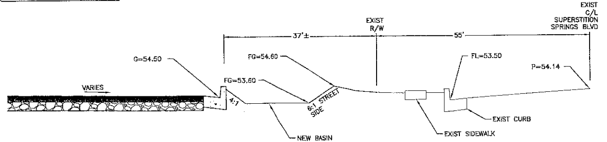
SECTION A-A NOT TO SCALE
